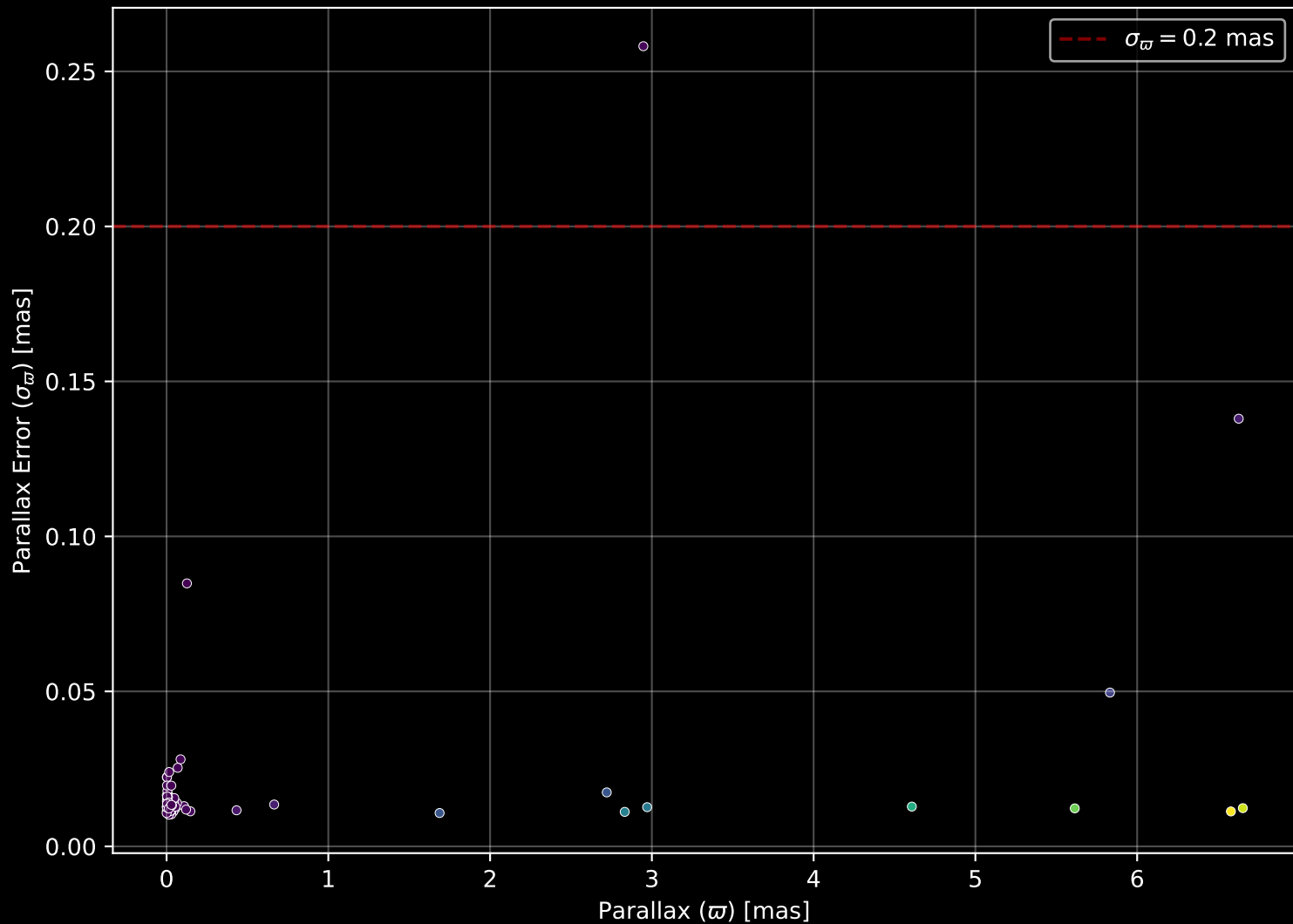
APOGEE DR17 Field: [303-44-O] Parallax Quality (n= 81)
