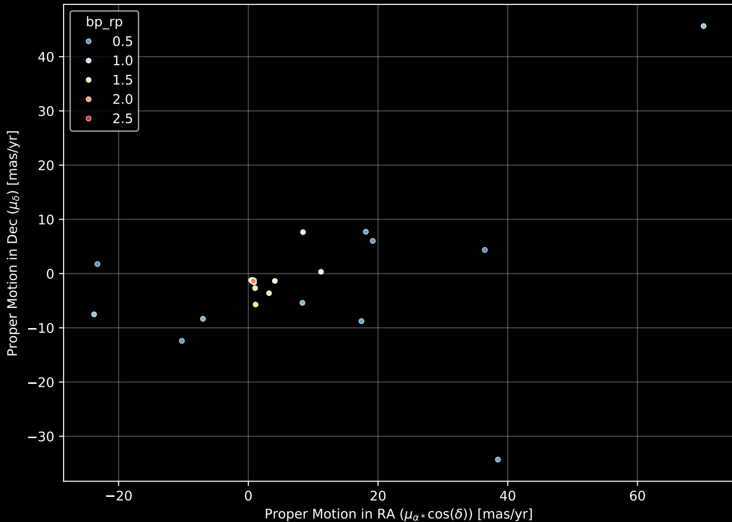
APOGEE DR17 Field: [303-44-O] Proper Motion Diagram (n= 81)
