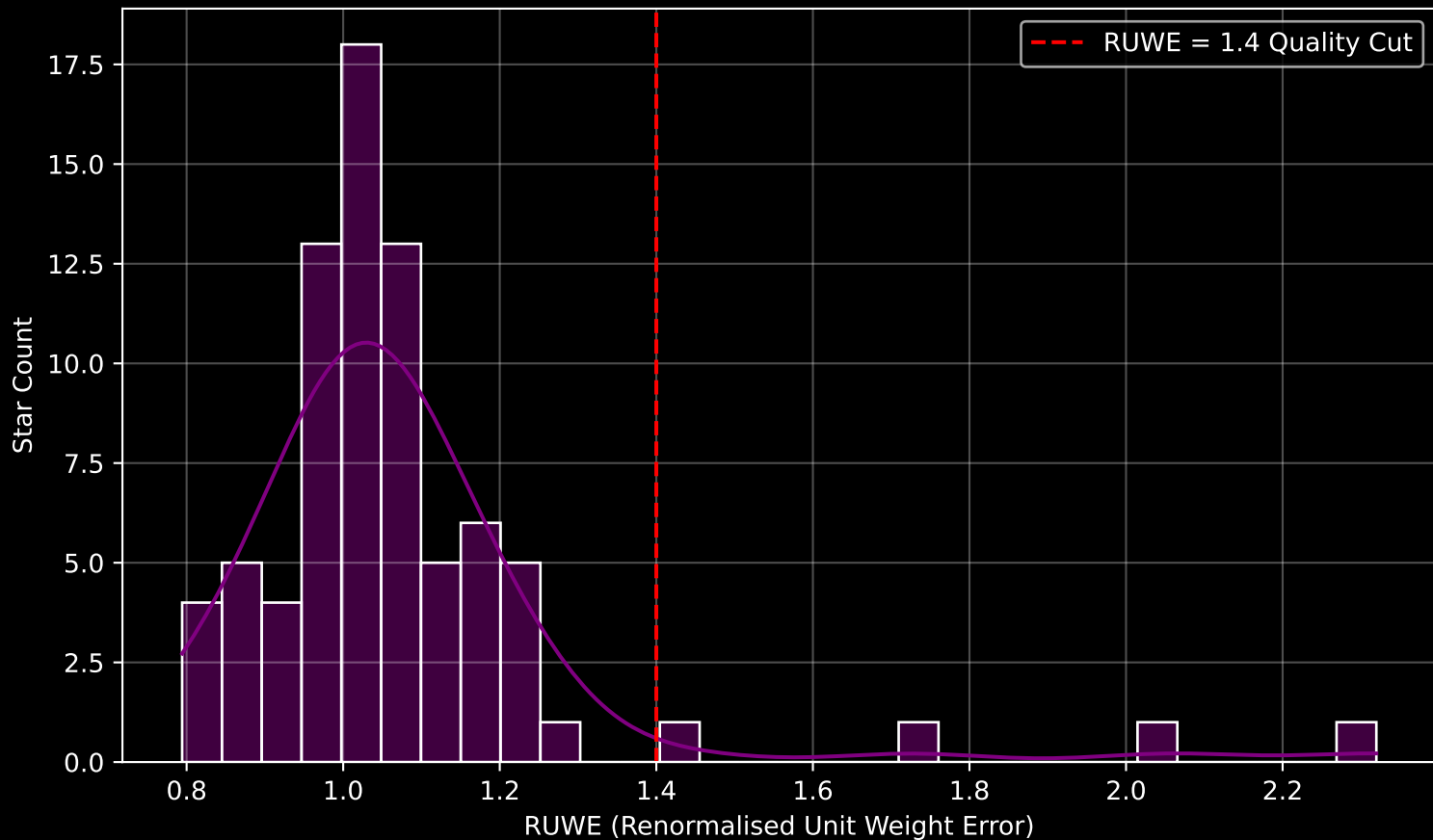
GAPOGEE DR17 Field [303-44-O] RUWE Distribution (n= 78)
