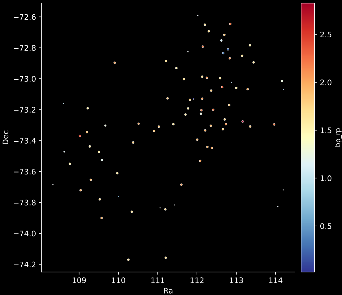
APOGEE DR17 Field: [303-44-O] Stars: 81
