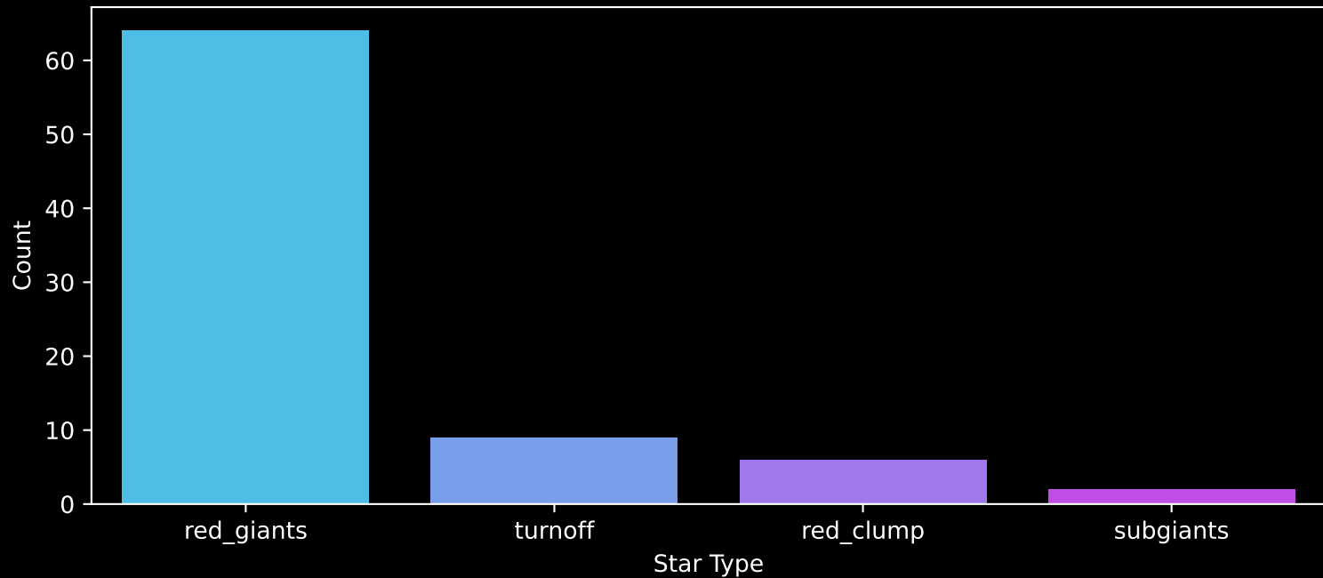
APOGEE DR17 Field: [303-44-O] Count plot of Star Type
