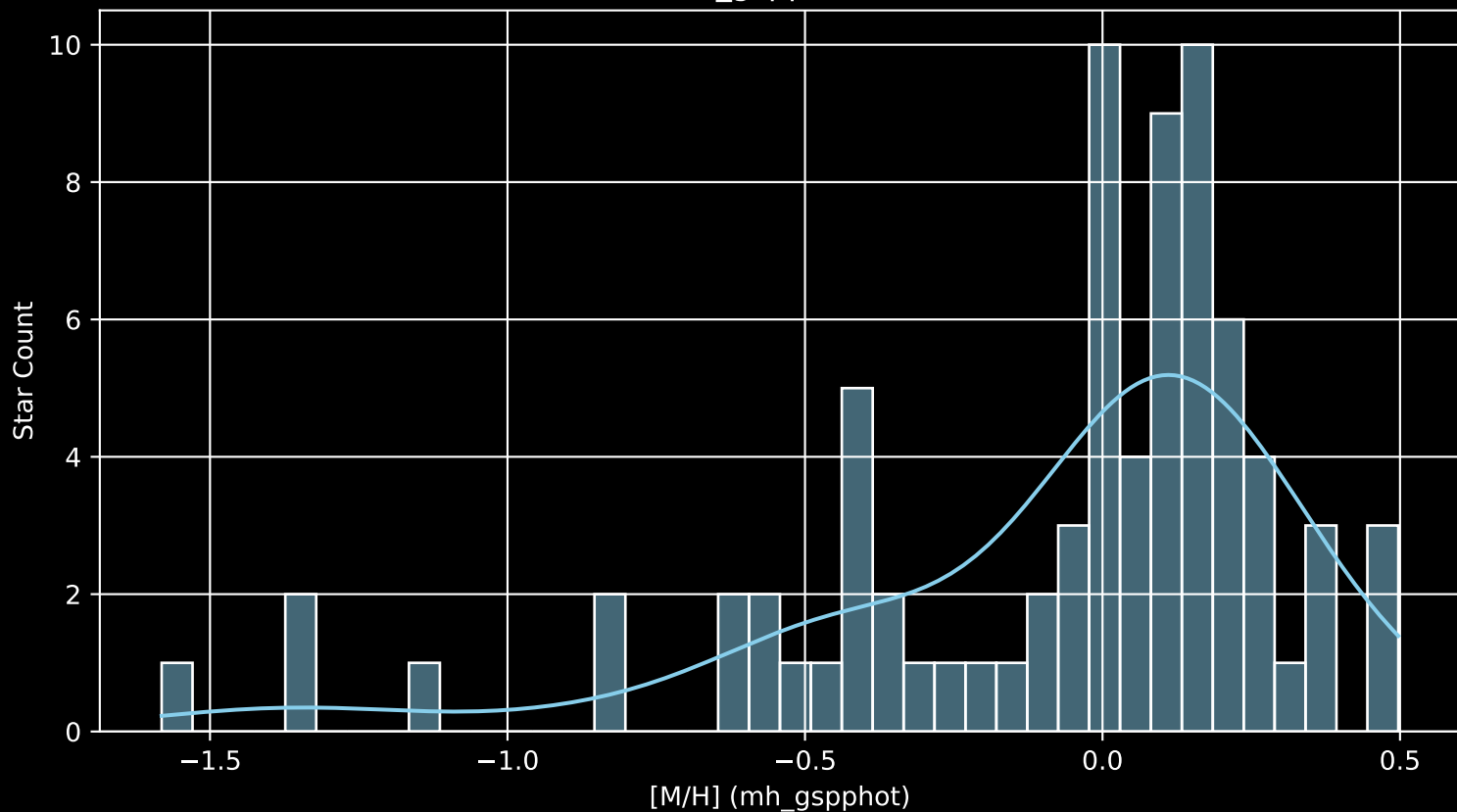
APOGEE DR17 Field: [303-44-O [M/H] (mh_gspphot) (n= 78)
