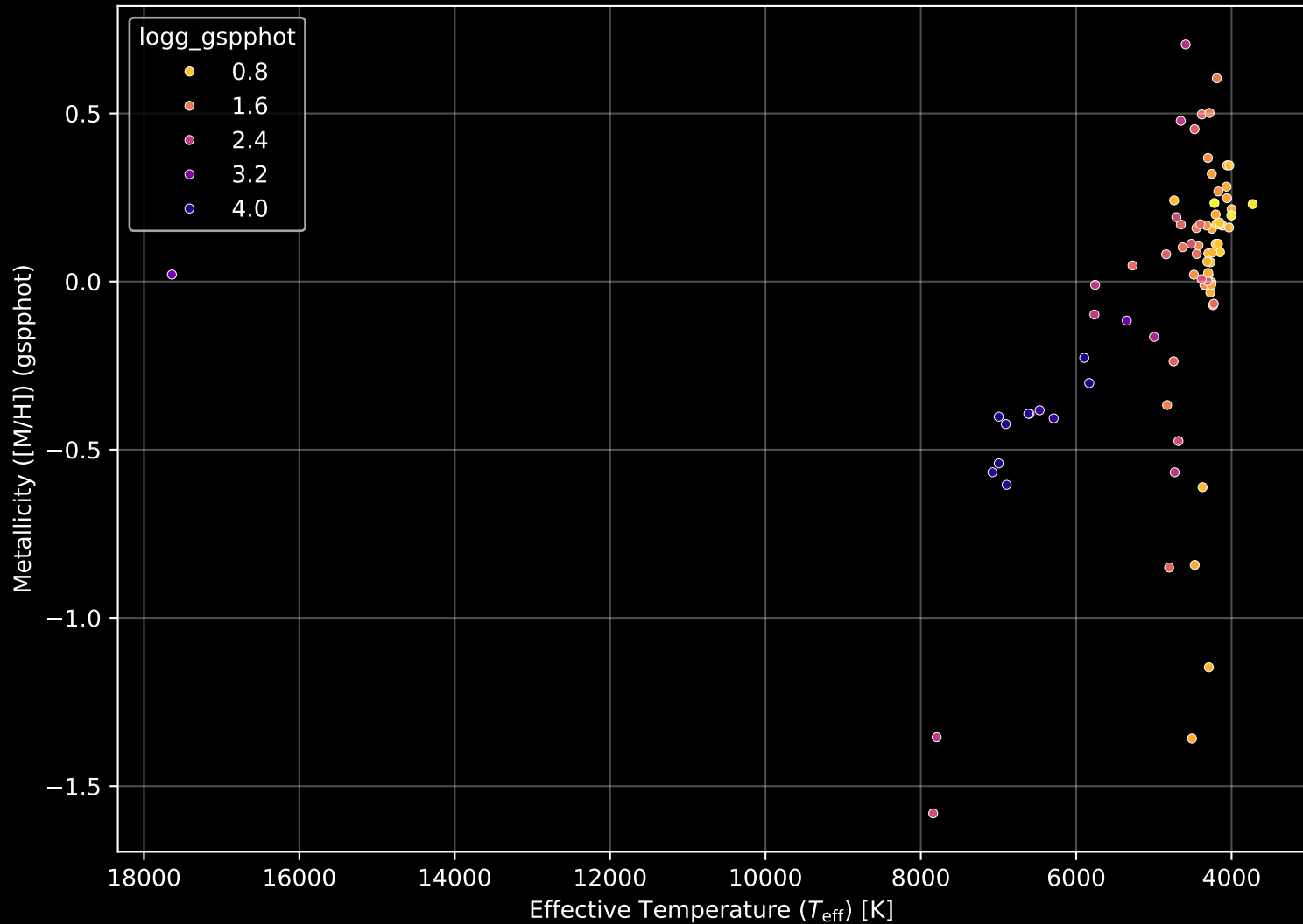
APOGEE DR17 Field: [303-44-O] Stellar Population Parameters (n= 81)
